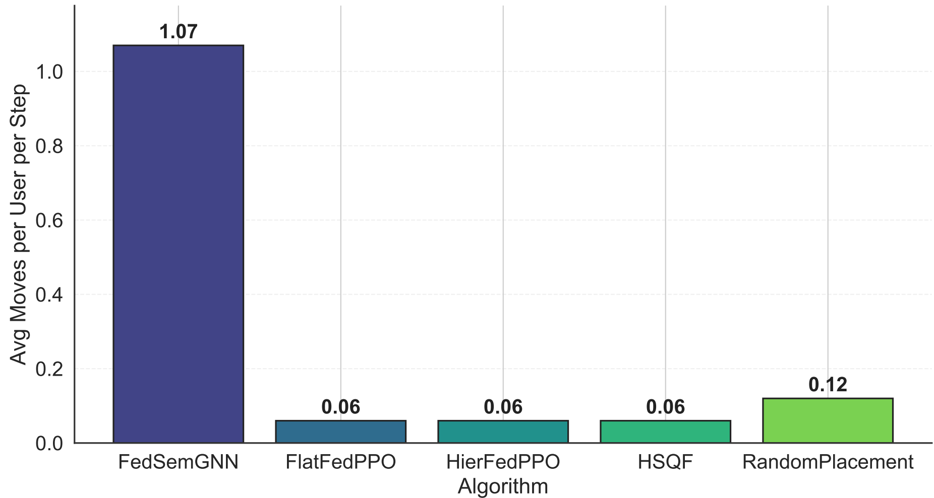
Average User Moves per Step (Mobility)
